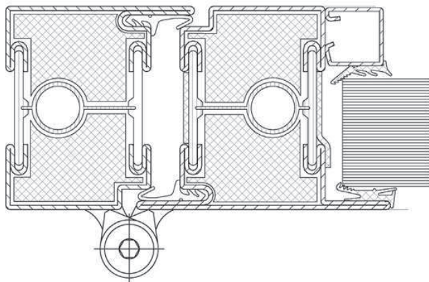
Jansen Janisol C4
